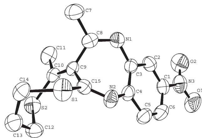
Figure 3. ORTEP drawing of 5 .
