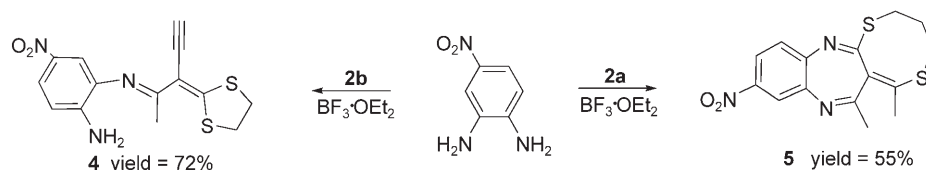
Scheme 2. Reaction of 4-nitro- o -phenylenediamine with 1,4-diynes 2a and 2b in the presence of BF 3 ·OEt 2 .
