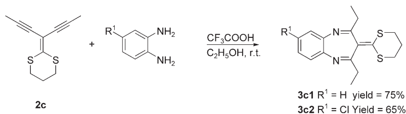
Scheme 3. Hydroamination of 2c with o -phenylenediamines.
