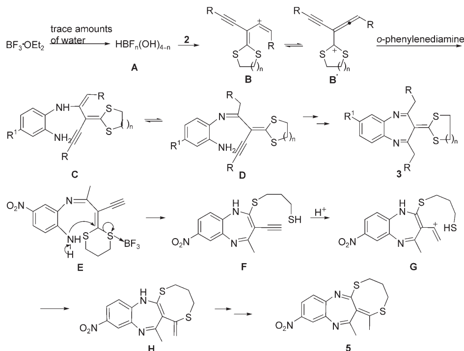
Scheme 4. Proposed mechanism for proton-catalyzed hydroamination reaction of diynes 2 .
