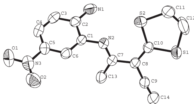
Figure 2. ORTEP drawing of 4 .
