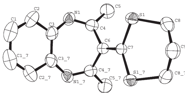
Figure 1. ORTEP drawing of 3a1 .
