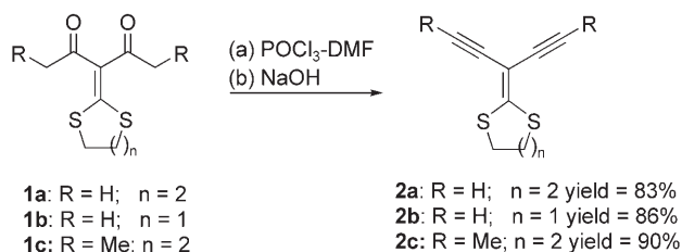
Scheme 1. Synthesis of \alpha,\alpha -dialkynylketene S,S -acetals 2 .
